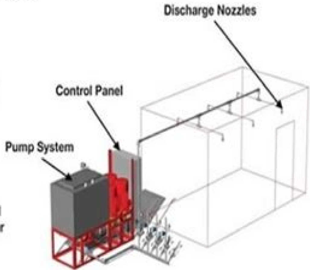
Watermist Total Flooding System
