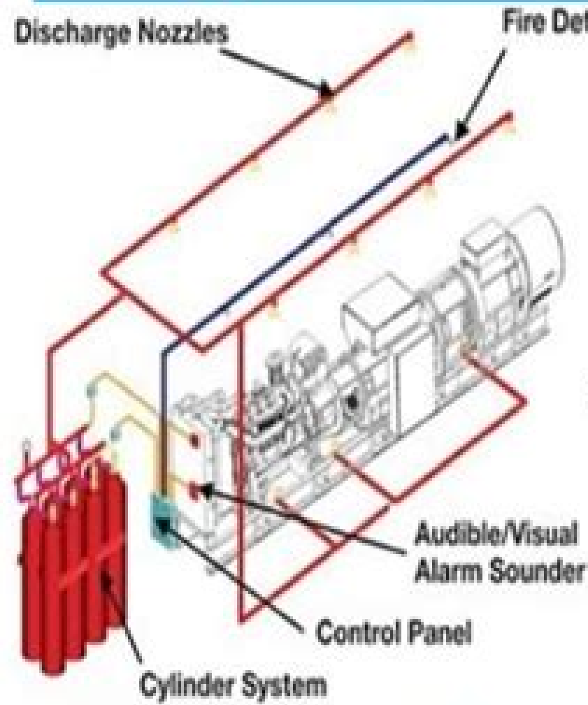
Watermist Local Application System
