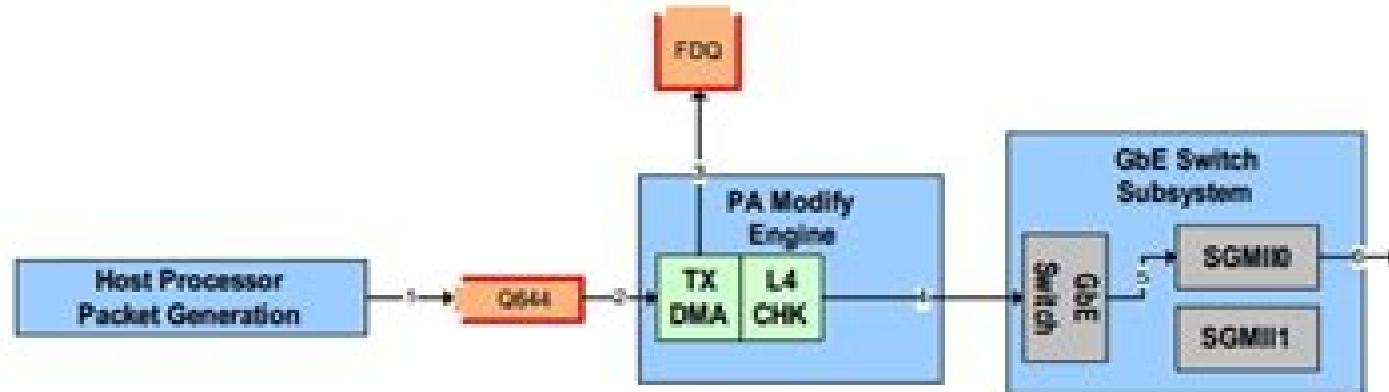
Figure 3-2 Transmit Checksum Generation Example
