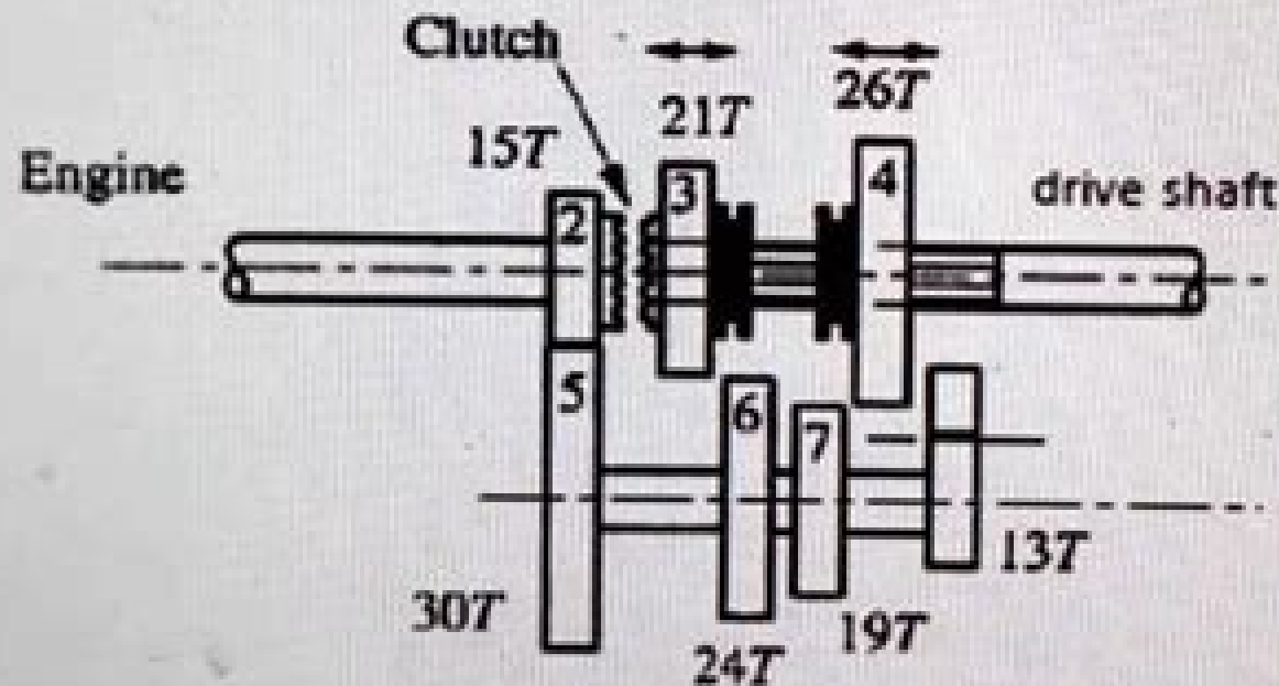
Figure Q1: Three-speed transmission system
