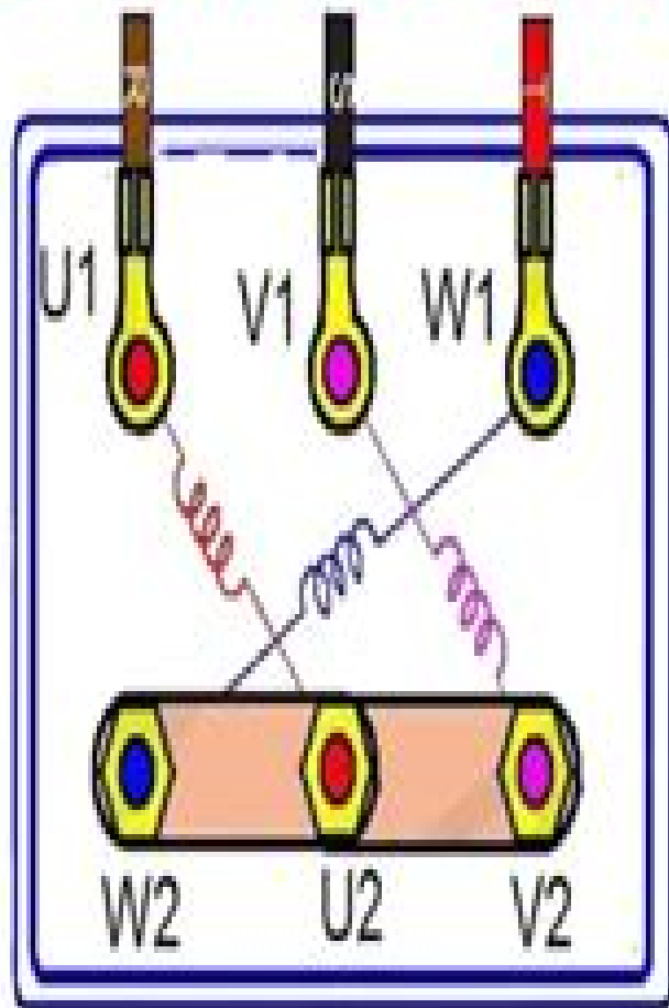
STAR CONNECTION
