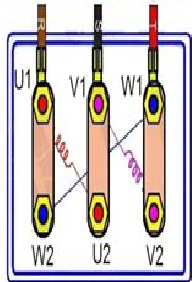
DELTA CONNECTION
