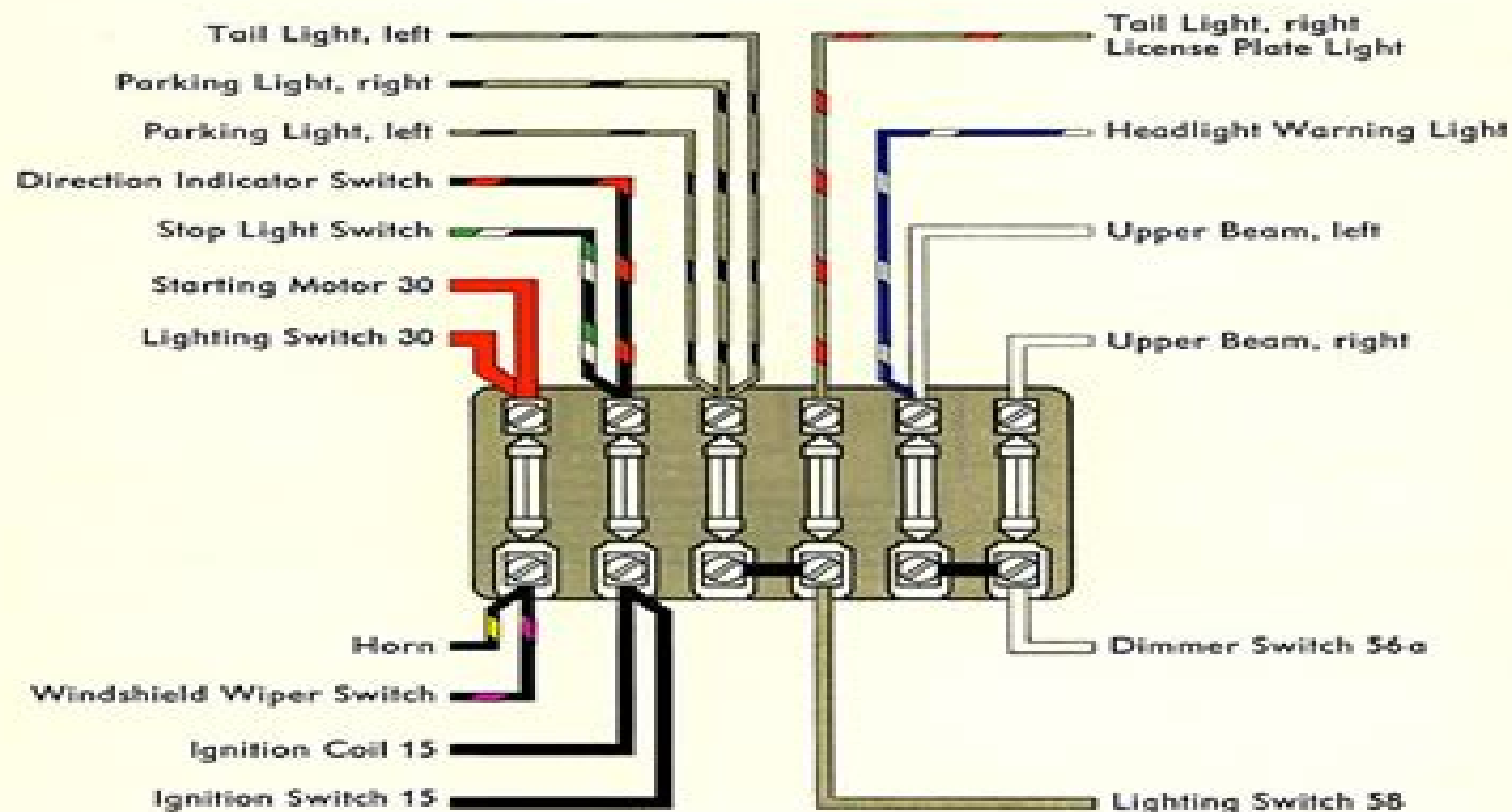
Fuse Box below instrument panel
