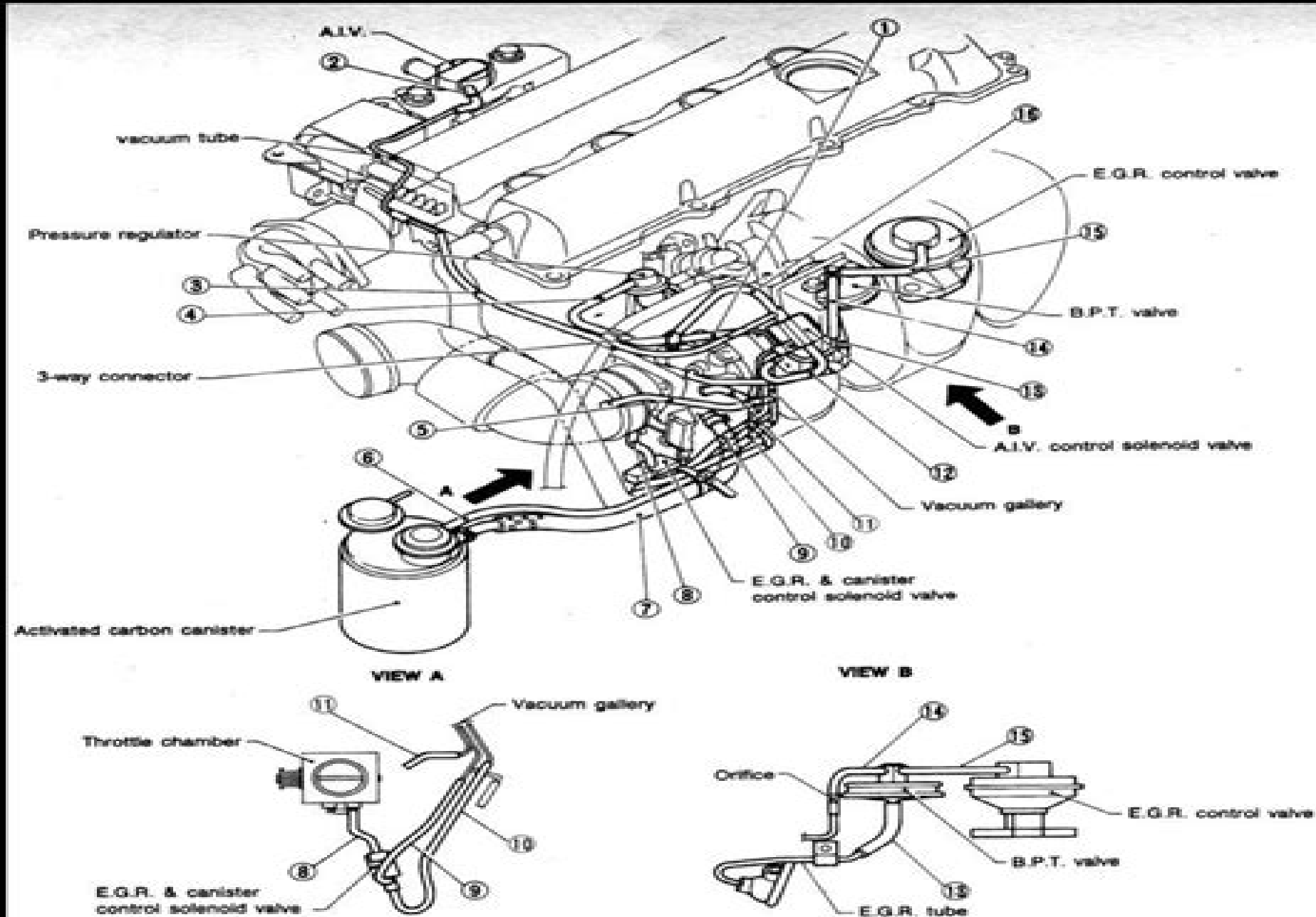
1.7n Vacuum hose routing diagram for 1991 through 1994 MPFI models with the SR20DE engine
