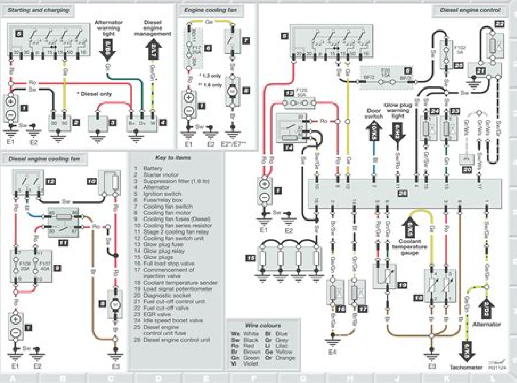
Diagram 2: Starting, charging, and Diesel engine control
