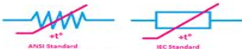
PTC Thermistor or Thermal Resistor Symbol
