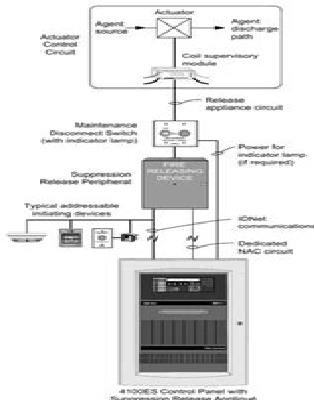
4100ES Series Releasing Control Typical Block Diagram
