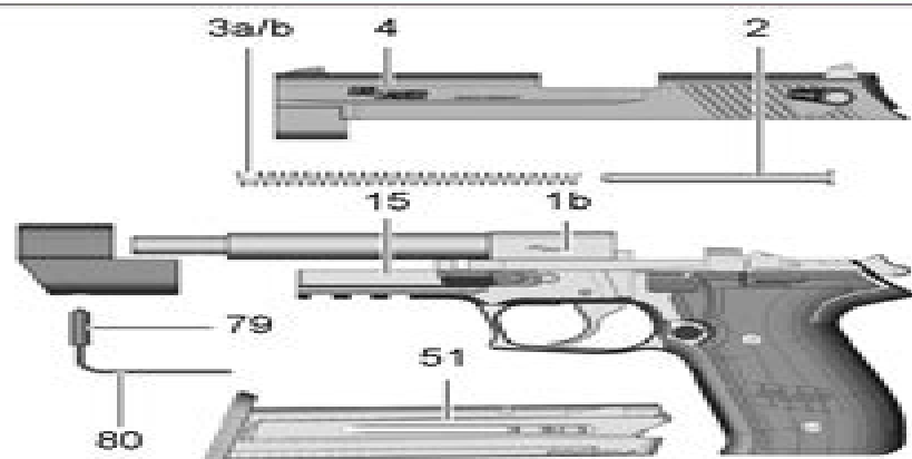
Fig. 18. Cleaning Sport version
