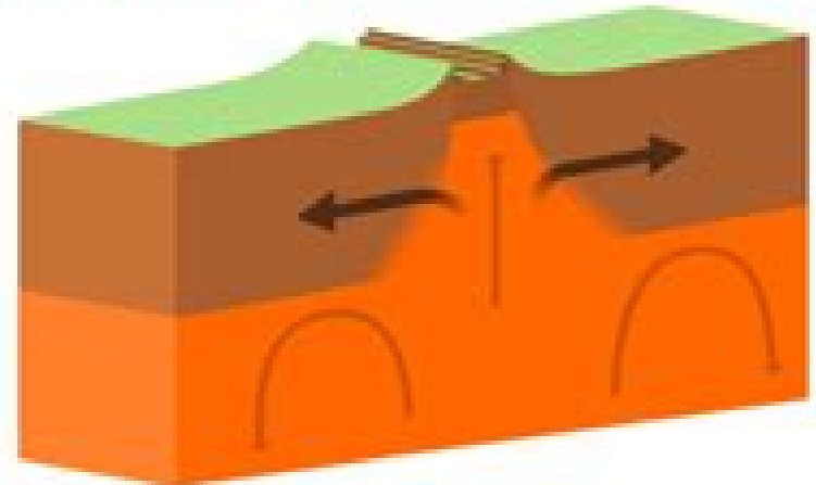
Divergent boundaries
