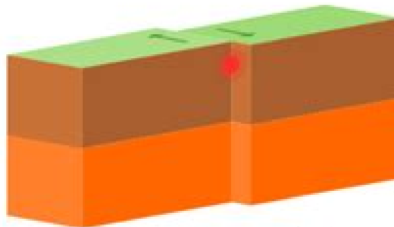
Transform boundaries
