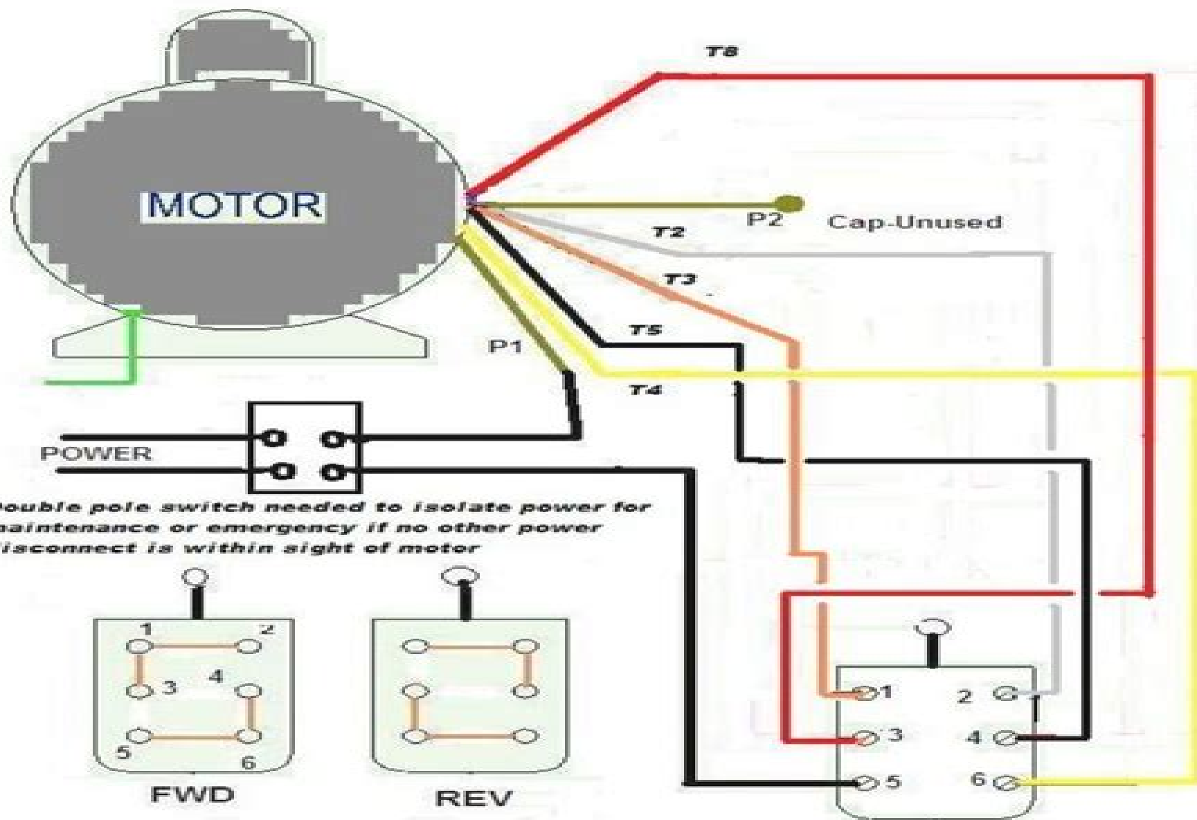
Contact configuration
