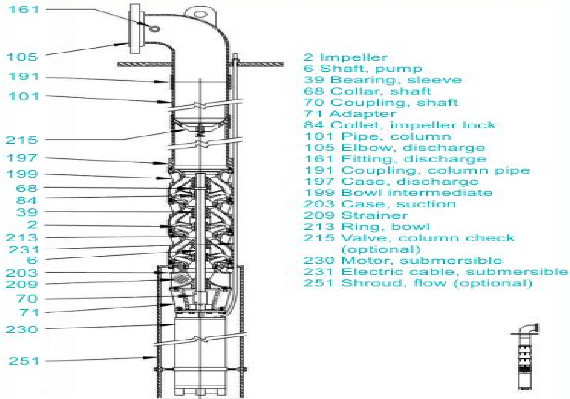
Vertical, Multistage, Submersible Pump
