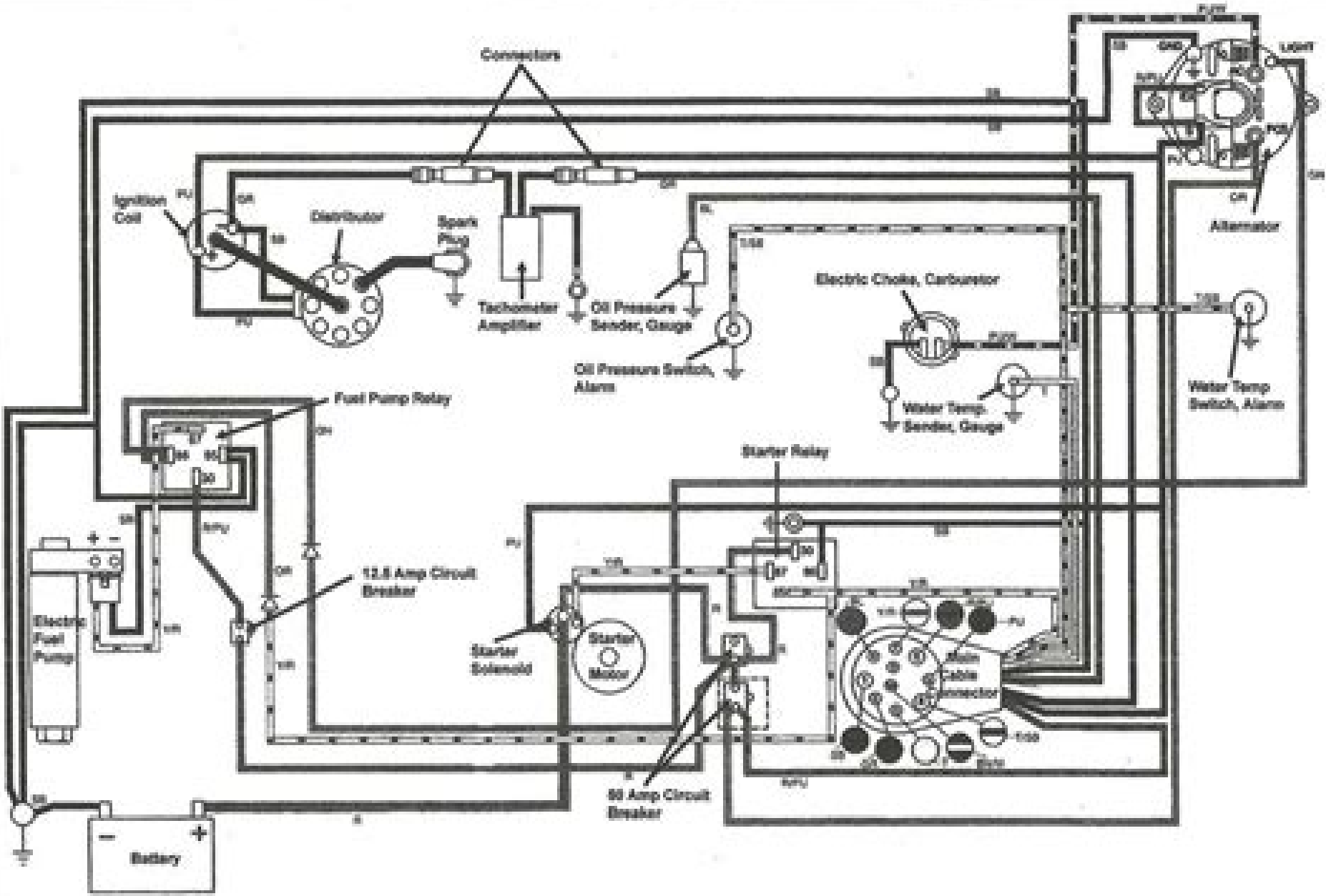
Fig. 206 Engine wiring schematic—1933-36 7.4L and 8.2L engines (carburetor)
