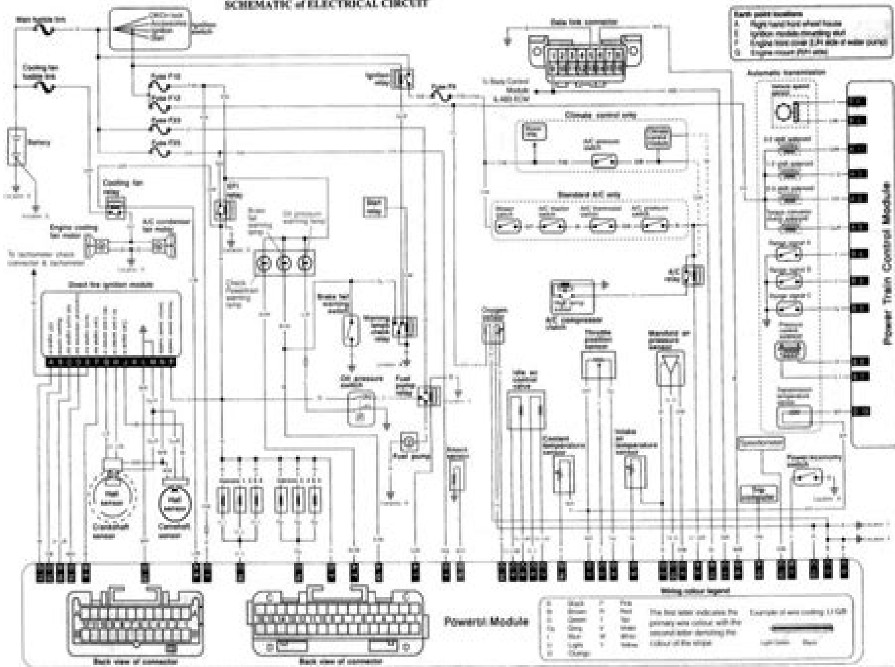
SCHEMATIC OF ELECTRICAL CIRCUIT
