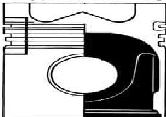
Figure 1 Piston for TD61 GD (principle diagram)
