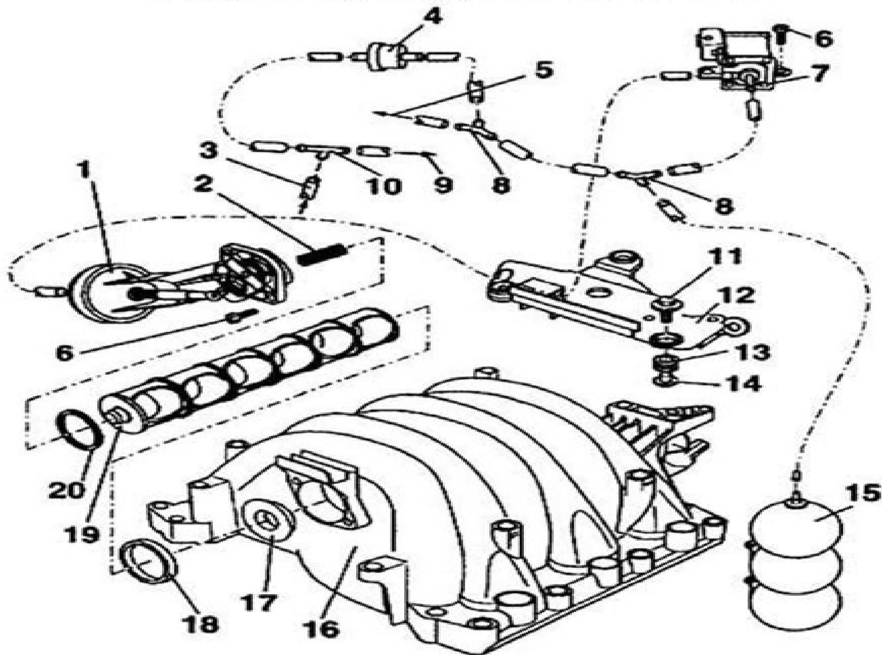
Fig. 26: Vacuum Diagram Intake Manifold Change-Over System (2.8L V6) Courtesy of VOLKSWAGEN UNITED STATES, INC.
