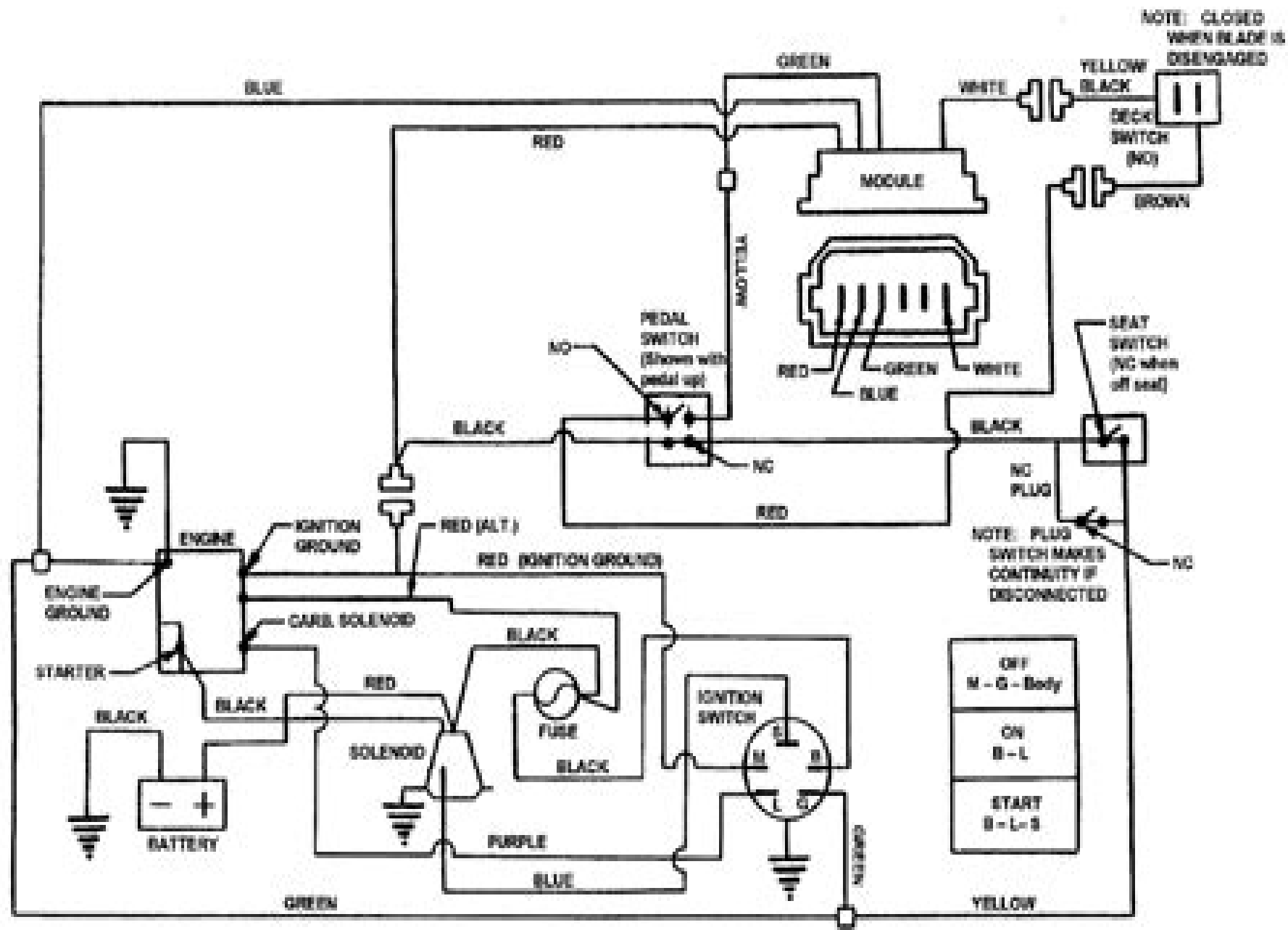
WIRING SCHEMATIC FOR 14.5 HP (BRIGGS ENGINE)
