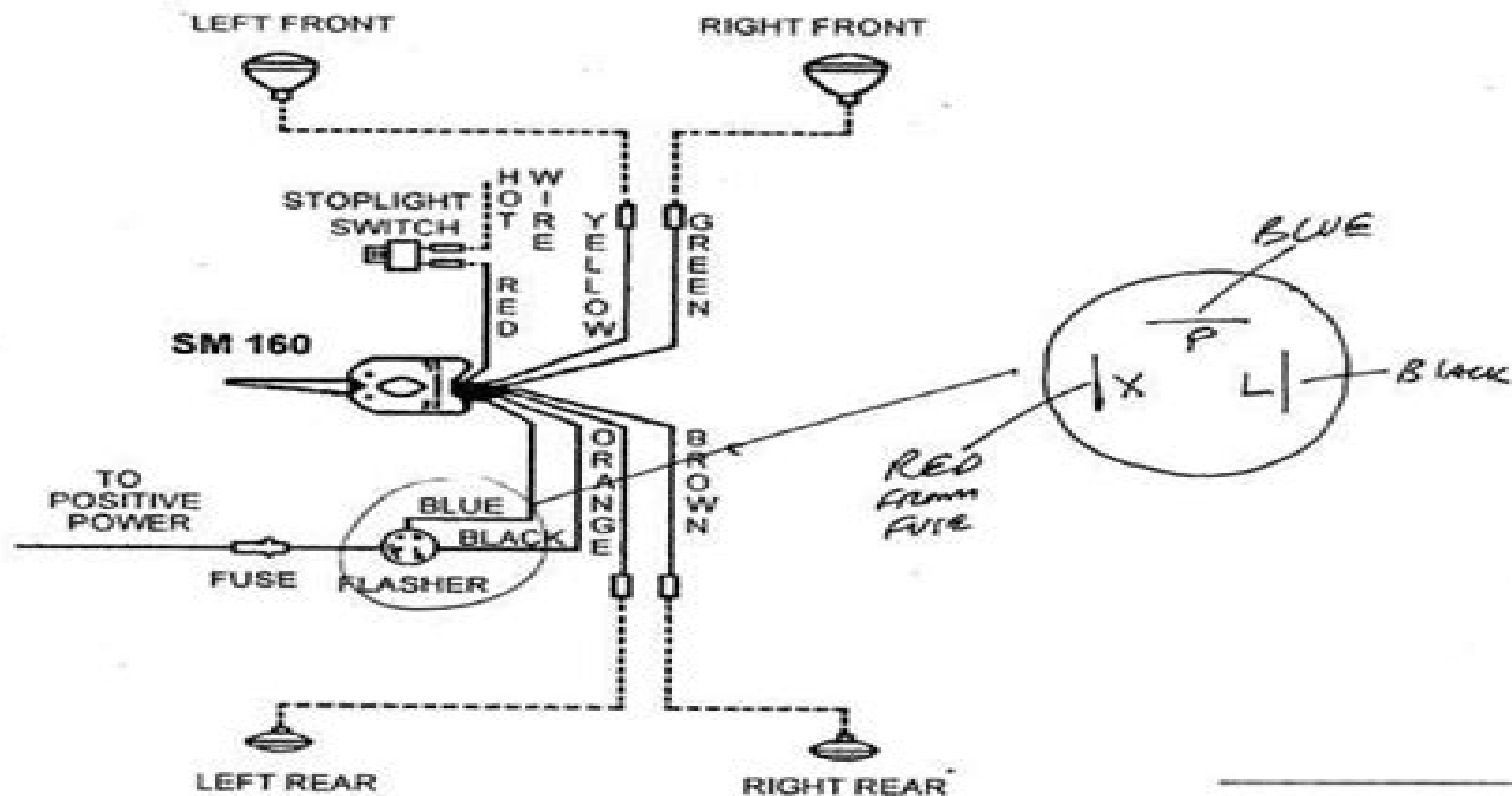
WIRING DIAGRAM
