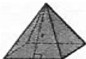
Regular Pyramid
