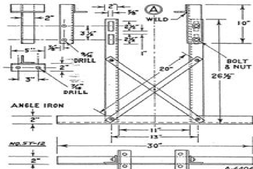
ILLUST. 128. CONSTRUCTION DETAIL OF THE HOME- MADE STAND WHICH SUPPORTS THE FRONT OF ENGINE
