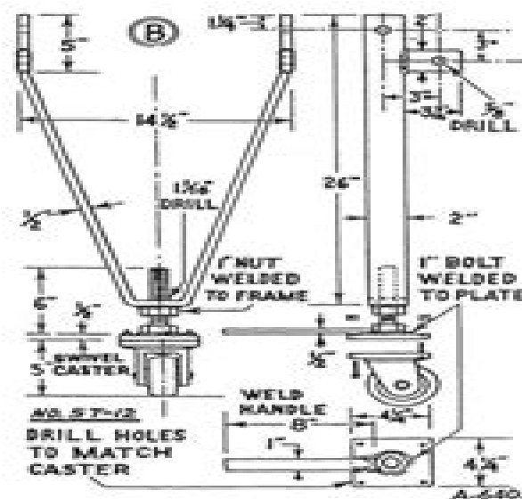
ILLUST. 18C. CONSTRUCTION DETAIL OF THE MOBILE PART OF THE TRACTOR SUPPORT WITH WHICH THE REAR SECTION OF THE TRACTOR IS BACKED AWAY FROM THE FORWARD OR ENGINE SECTION.
