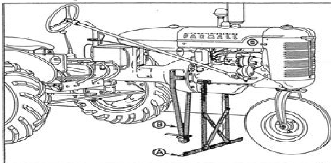
ILLUST. 18A. SHOWING A SIMPLE METHOD OF SUPPORTING A FARMALL A OR B TRACTOR WHILE SEPARATING THE FRONT AND REAR SECTIONS FOR THE PURPOSE OF REMOVING THE CLUTCH.
