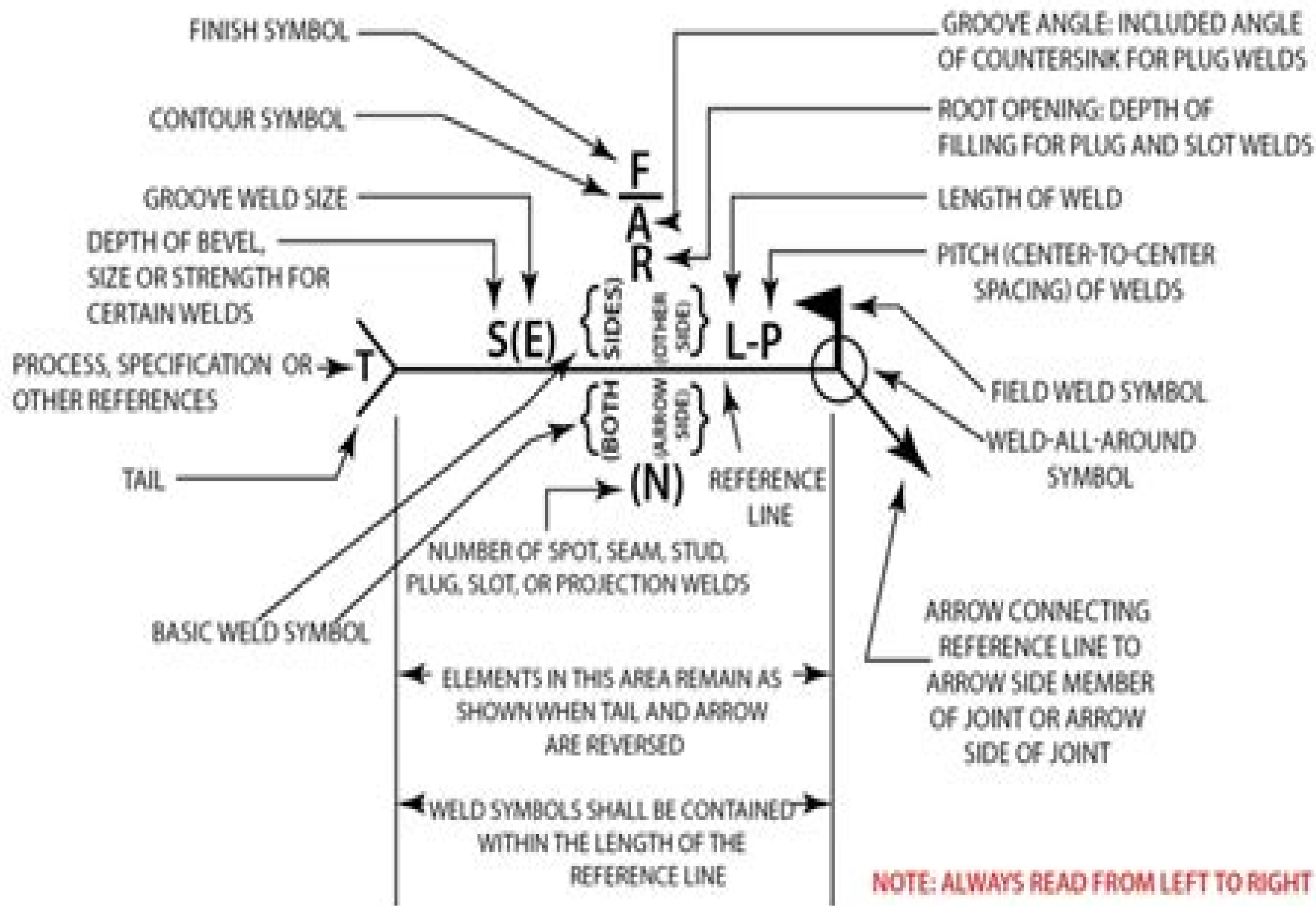
SCHEMATIC FOR ELEMENTS OF A WELDING SYMBOL WITH THEIR STANDARD LOCATIONS
