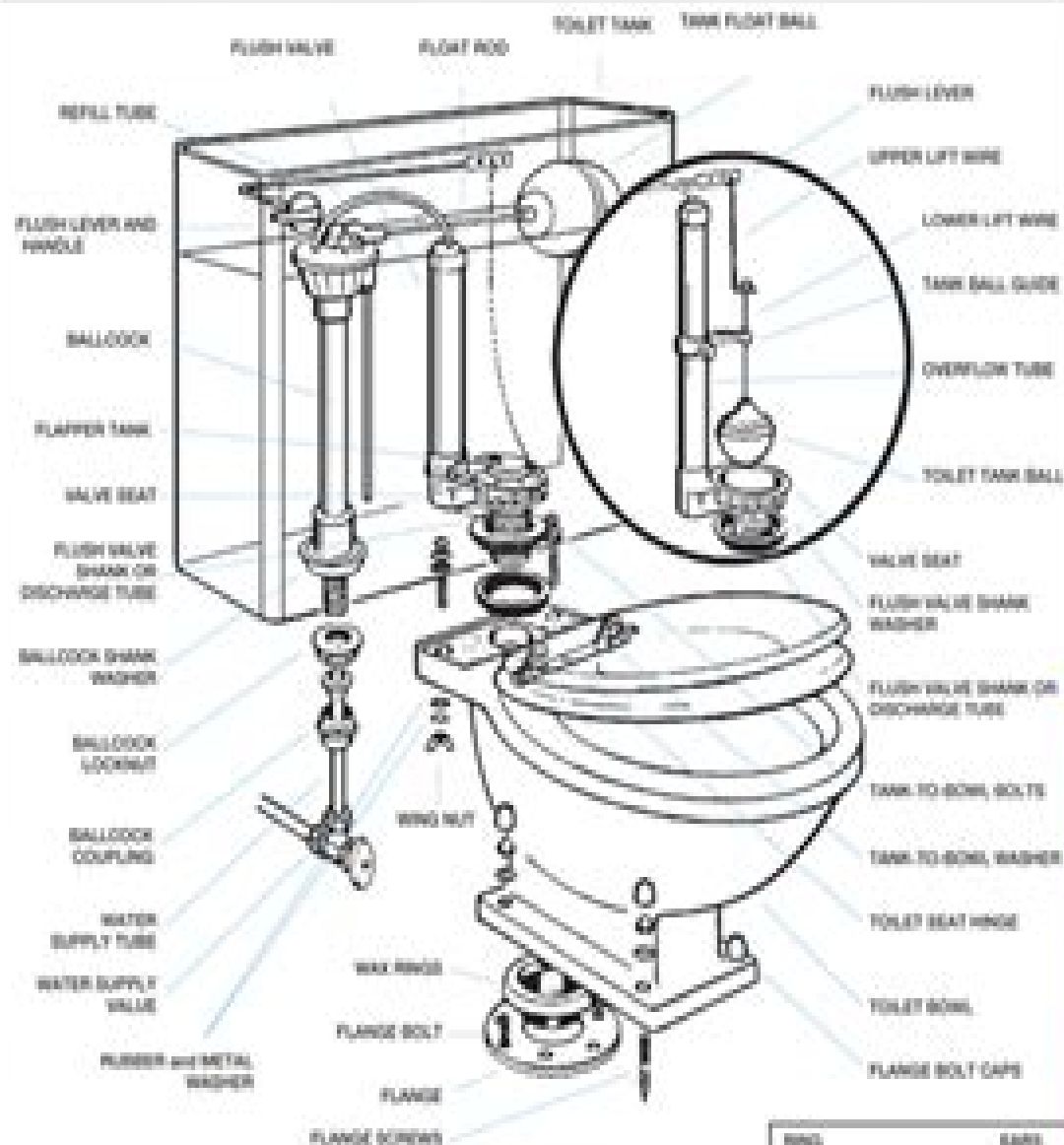
Homedit.com - Parts of a Toilet Diagram
