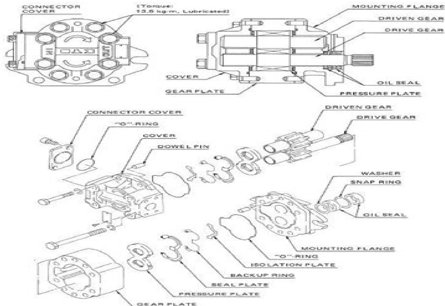
Fig. 41.35 Steering Pump Construction & Component Parts (850)
