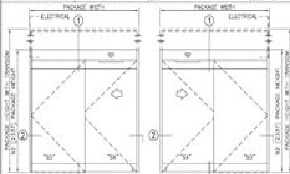
LEFT HAND SIDE ELEVATION VIEW RIGHT HAND SIDE SCALE: 1/8" = 1'-0"
