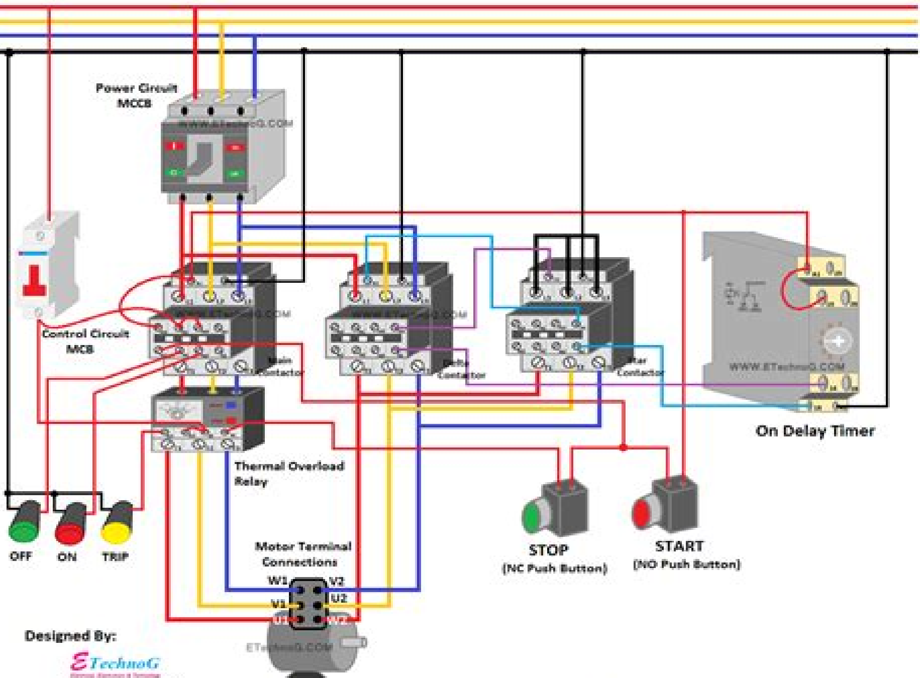
Star Dela starter Connection Diagram
