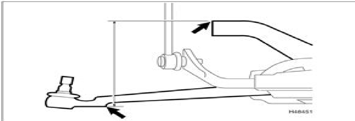
6.16 Raise the lower arm so the distance between the lower edge and the subframe upper edge is 187 mm
