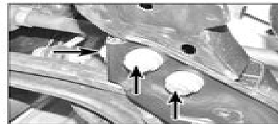
6.5 Undo the bolts (arrowed) and remove the subframe extension strut
