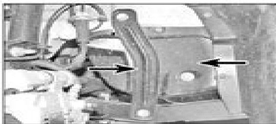
6.3 Remove the support bracket and wheel arch liner panel (arrowed)
