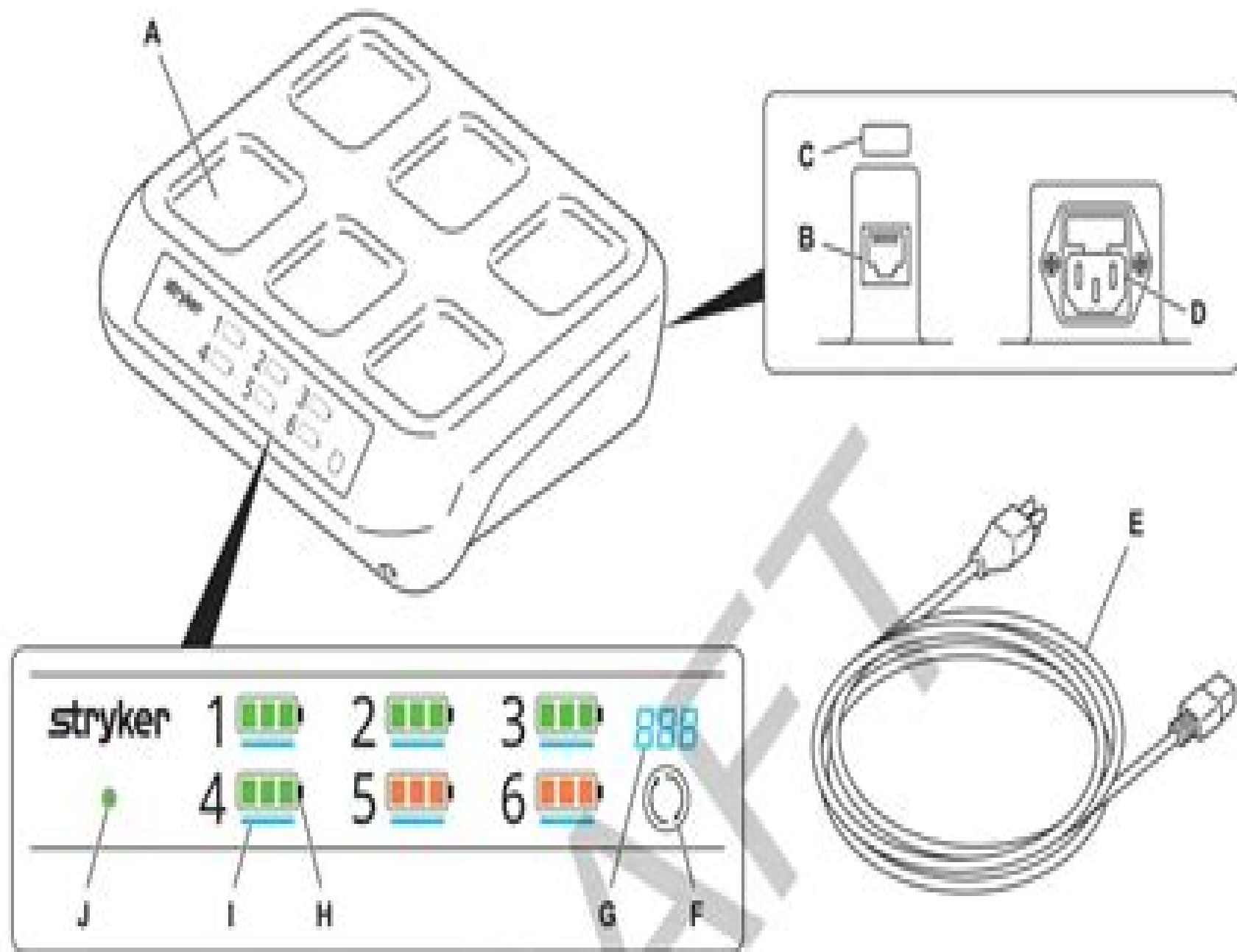
Figure 1 - Charger features
