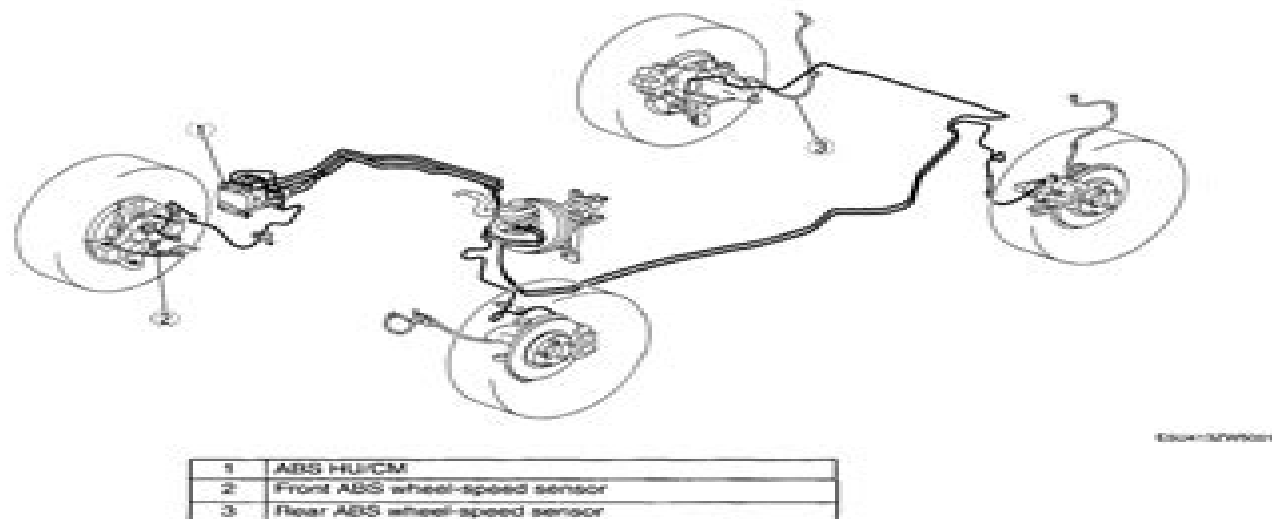
Fig. 1: Identifying Location Of ABS Components Courtesy of MAZDA MOTORS CORP.
