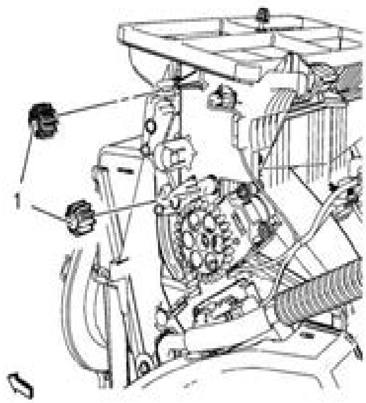
Fig. 28: Mode Valve Gear Courtesy of GENERAL MOTORS COMPANY
