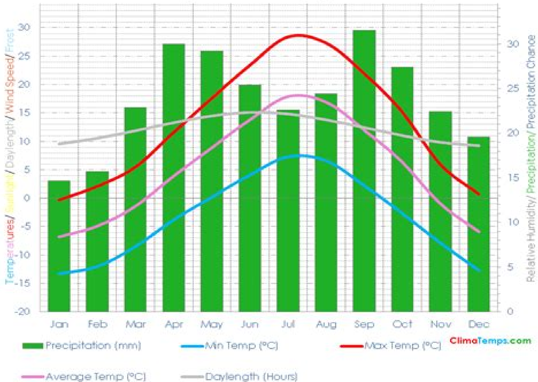
Evanston, Wy, Usa Climate Graph (Altitude: 2043 m)
