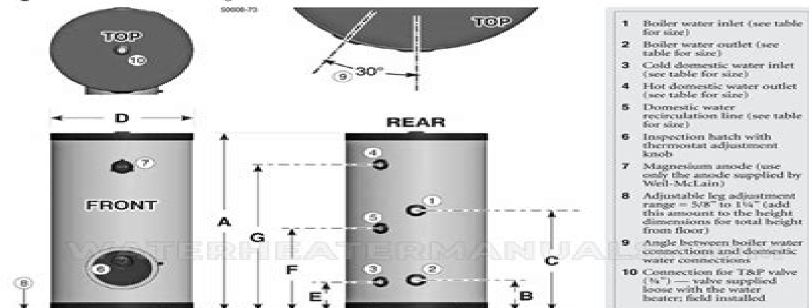
Figure 25 Dimensions and ratings — AQUA PLUS indirect-fired water heaters
