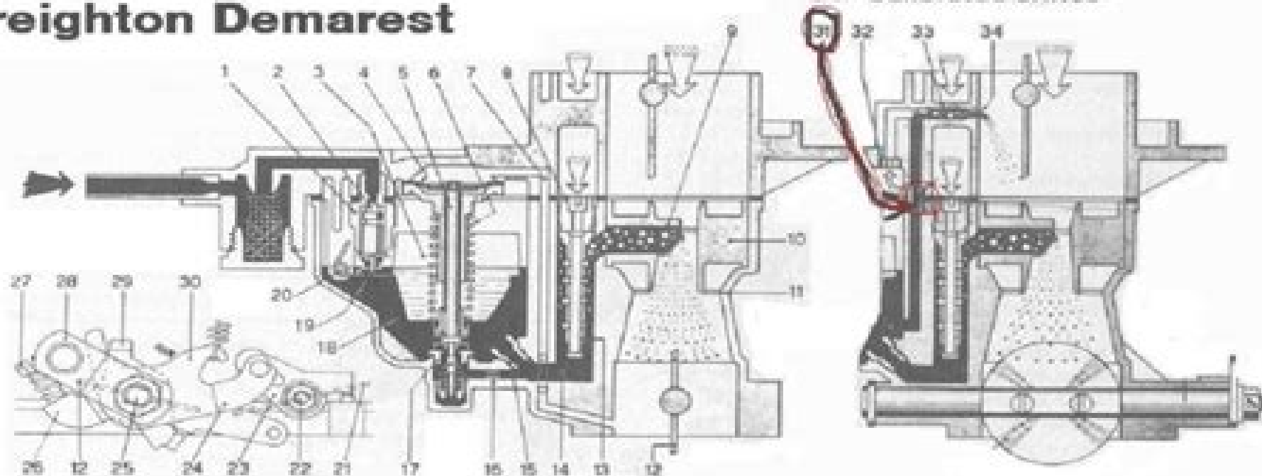
Fig. 7.6 Carburettor normal phase (Sec 3)
