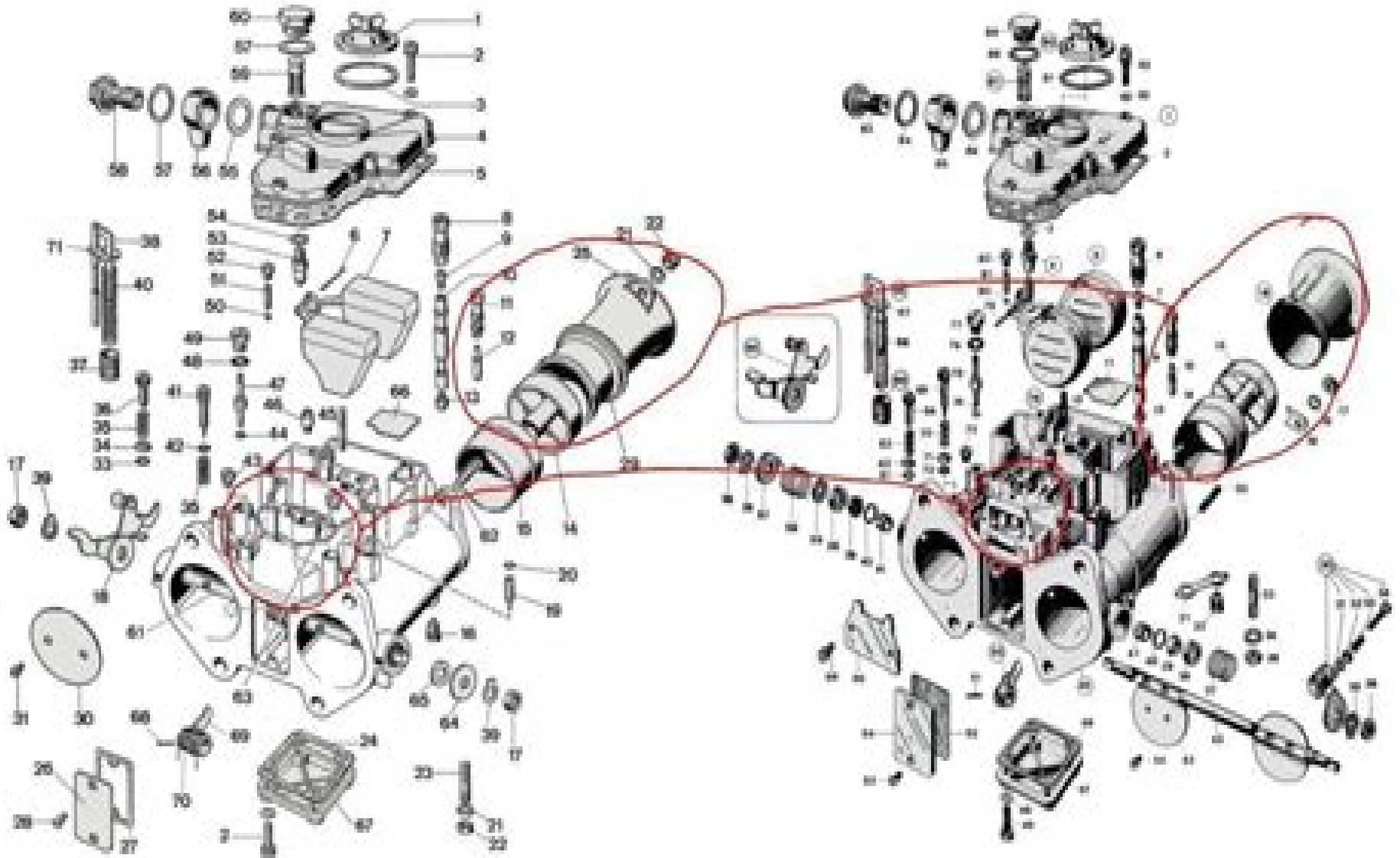
WEBER 48 DCO SP - exploded view
