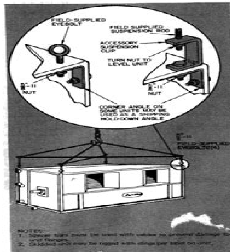
Fig. 1 — Rigging and Suspension Details
