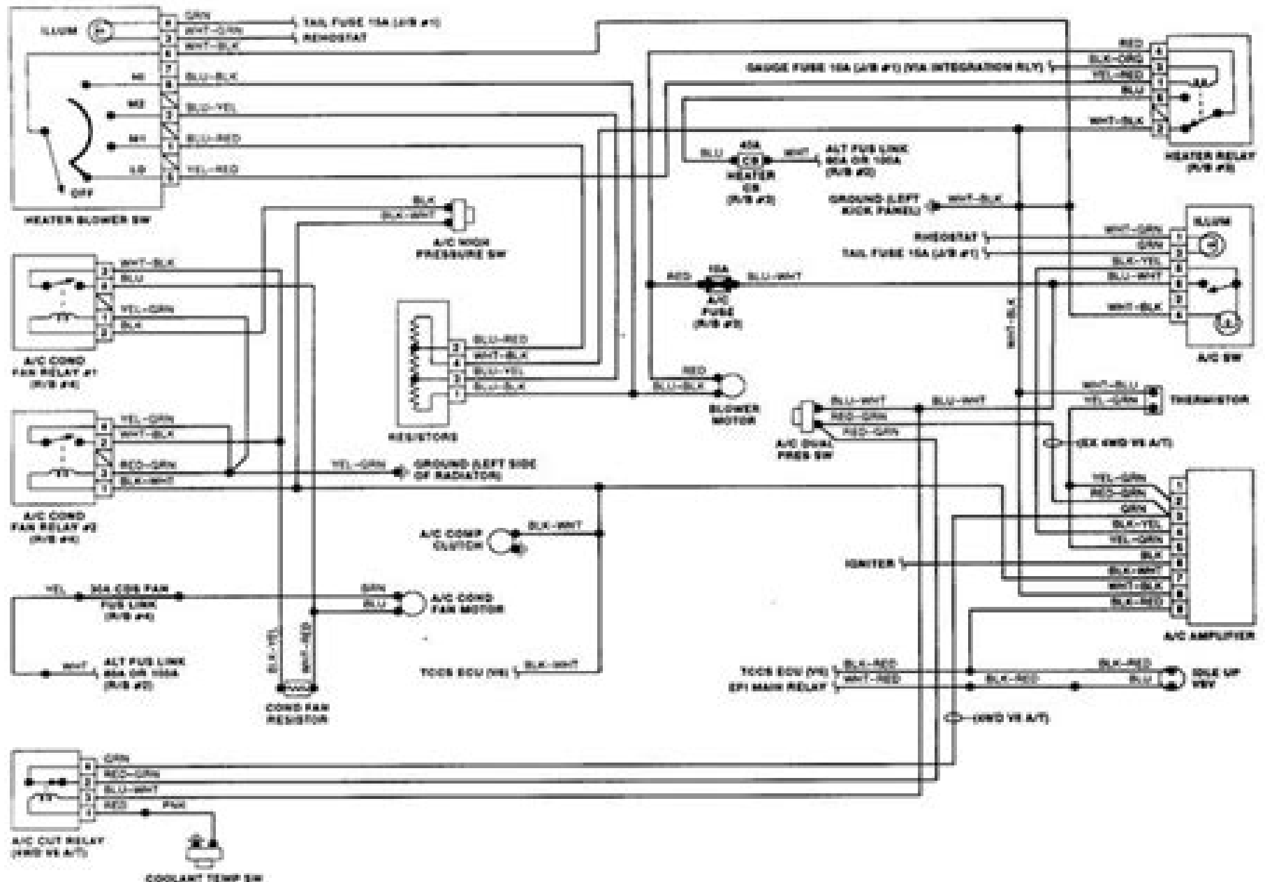
Fig. 17: Manual A/C-Heater System Wiring Diagram (4Runner)
