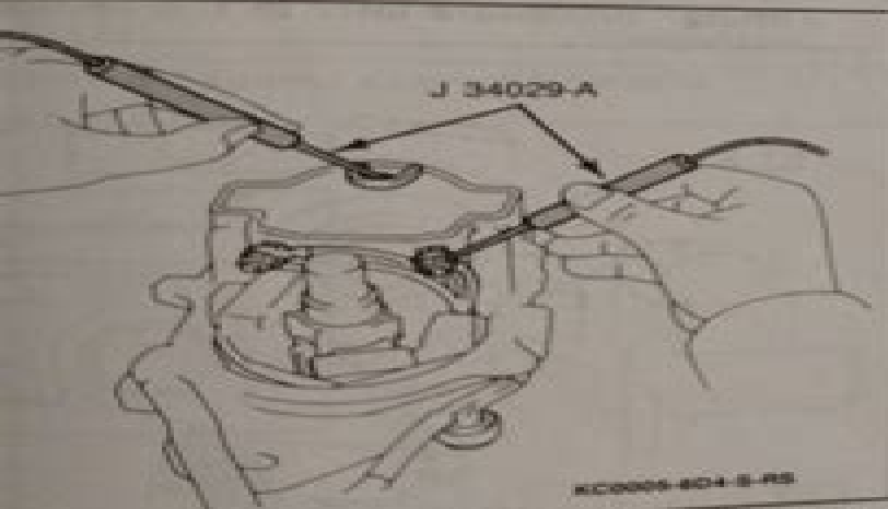
Measuring Secondary Ignition Coil Resistance
