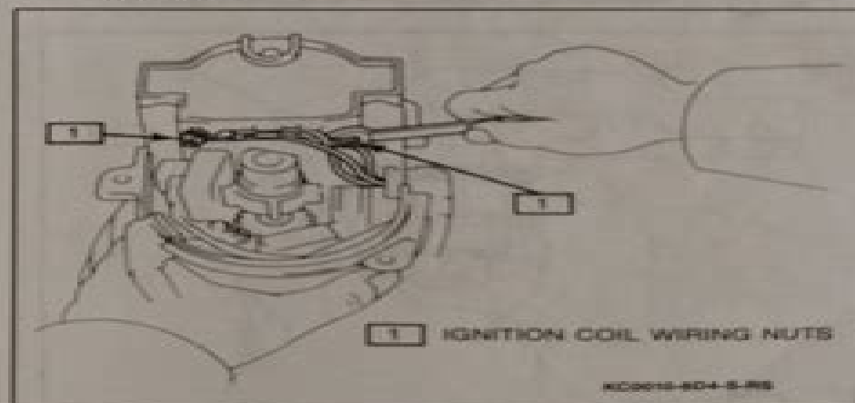
Figure 10 Removing Ignition Coil Wiring
