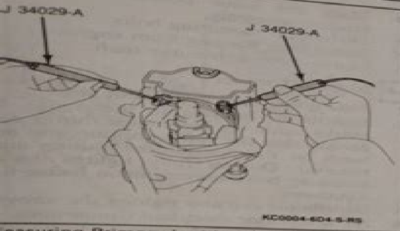
Measuring Primary Ignition Coil Resistance
