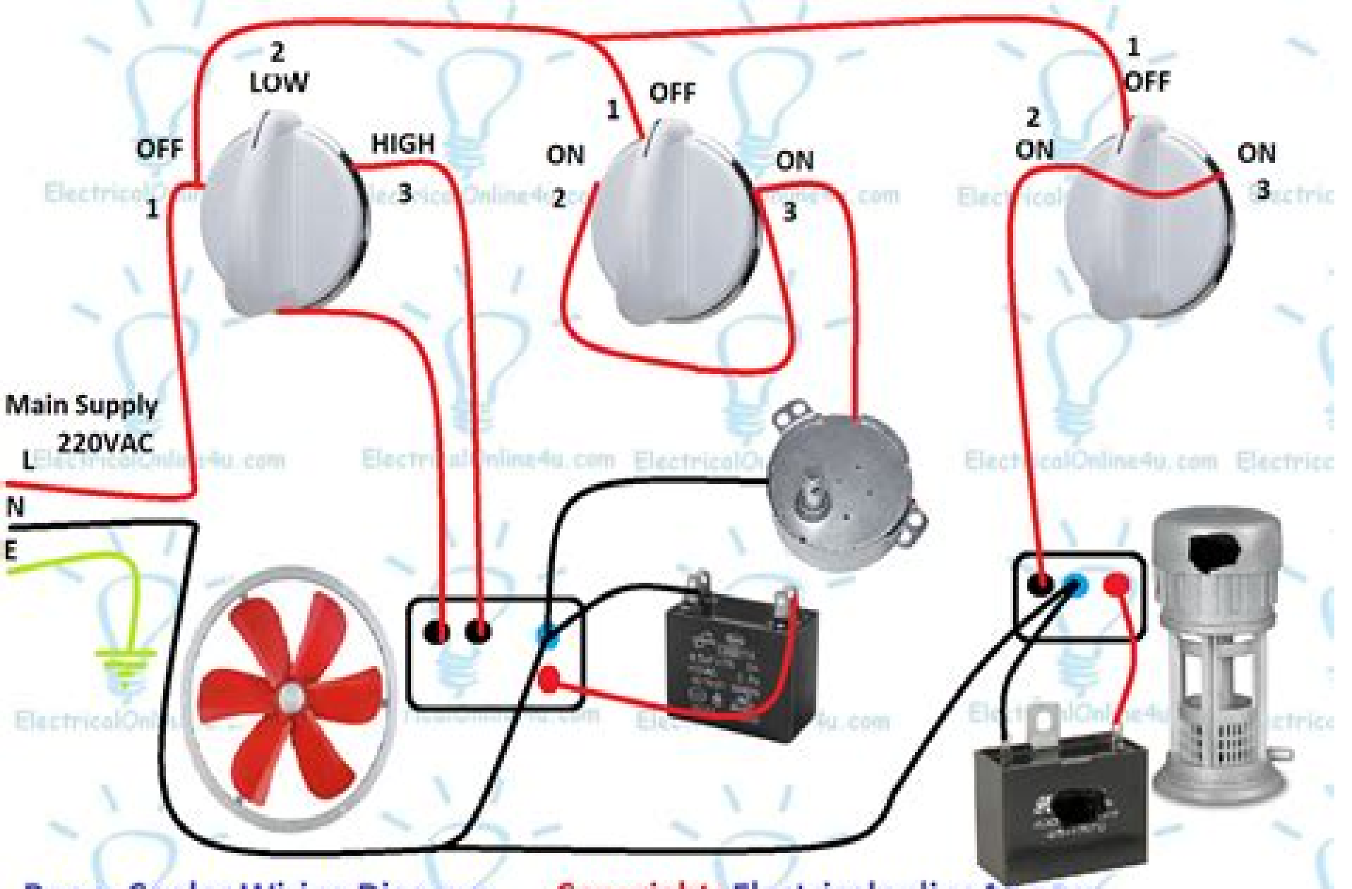
Room Cooler Wiring Diagram
