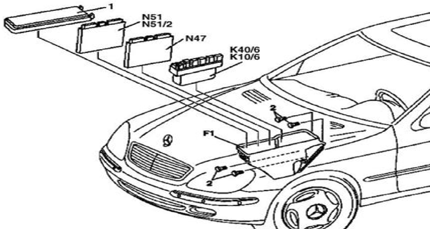
Fig 2: Identifying Location Of Fuse & Relay Box K40/6 As-Built Configuration
