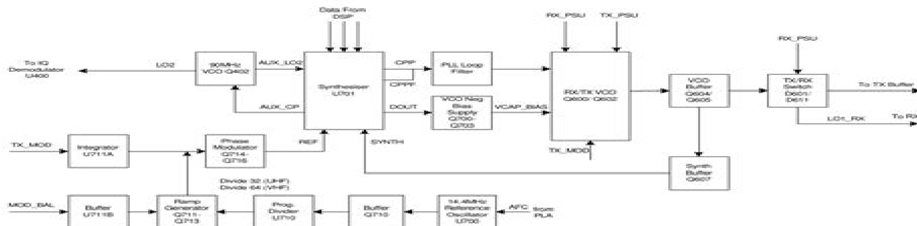
Figure 3-3 VHF/UHF Synthesiser, Block Diagram
