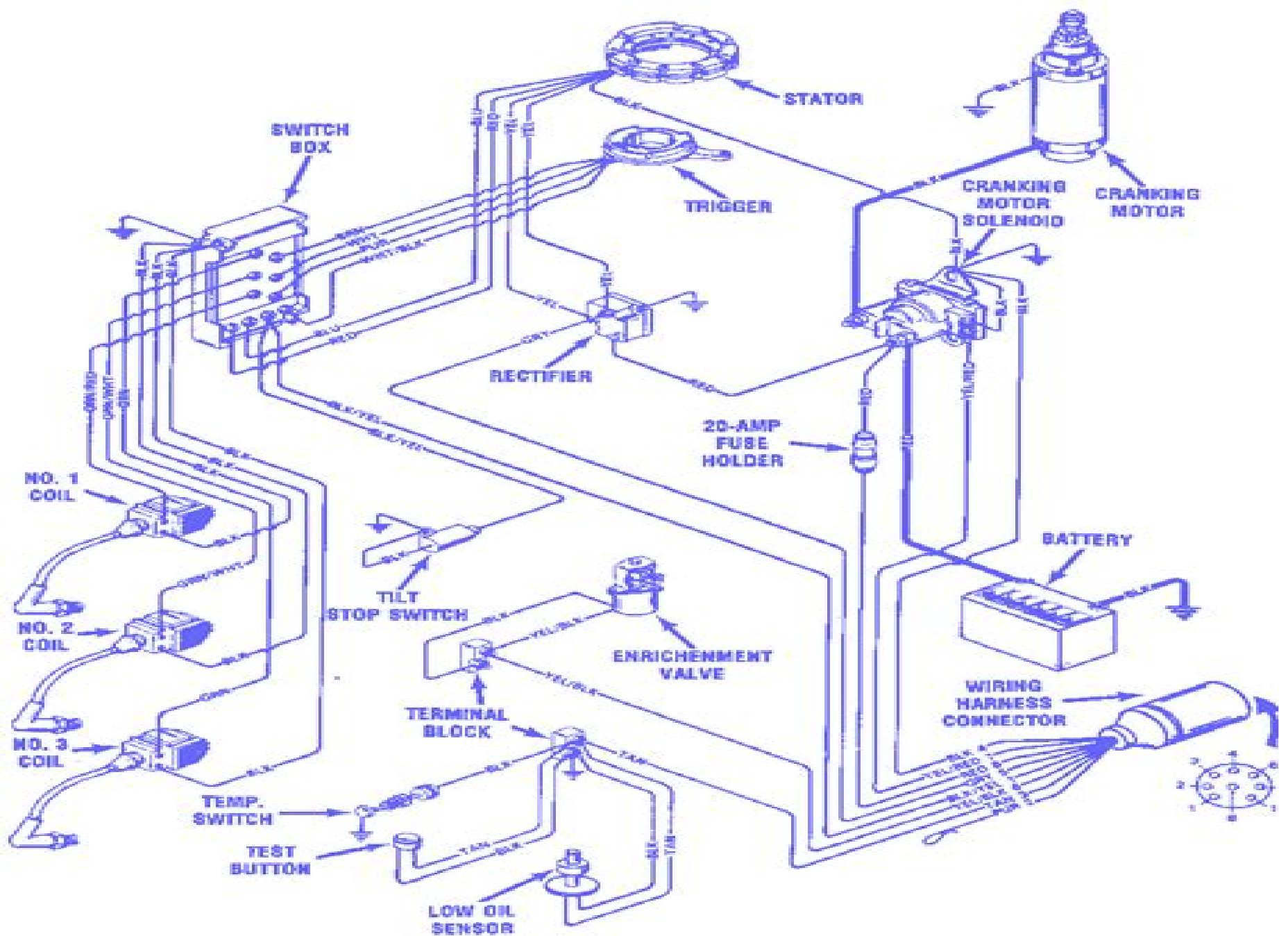
Functional wiring diagram for the 3-cylinder Model 76 and 90hp powerheads WITHOUT low oil warning module. Wire color code identification is indicated.
