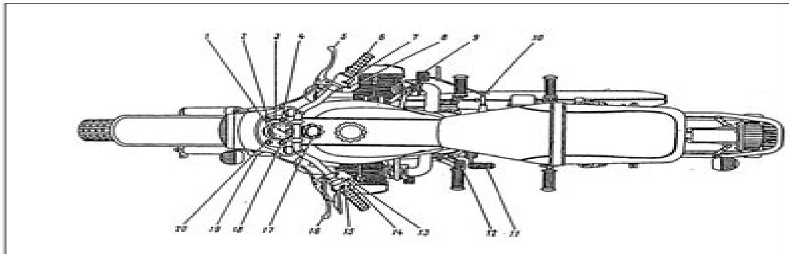
Figure 2.2-1. Controls and Instrumentations
