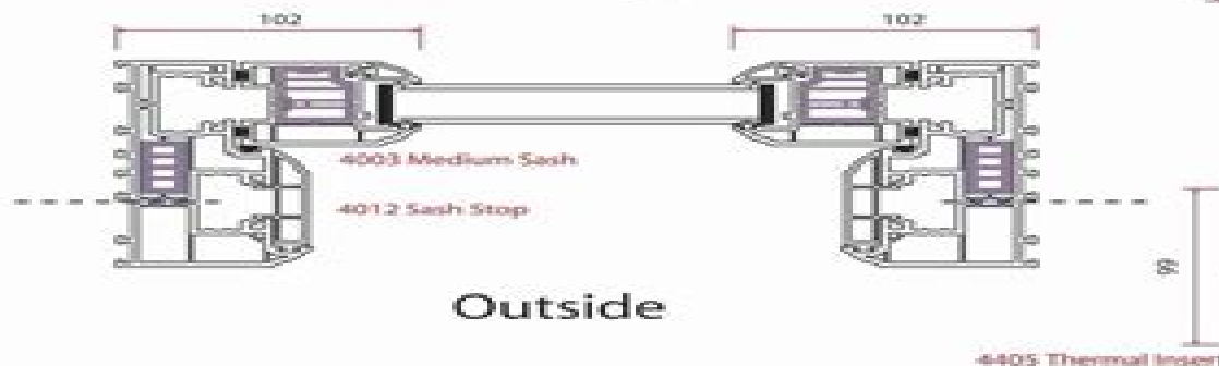
Horizontal section through bottom sash
