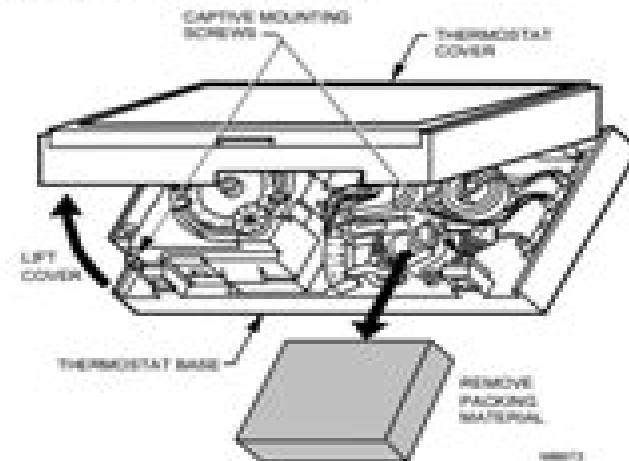
Fig. 1—Unpack thermostat.
