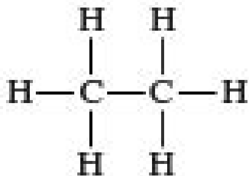
alkane
