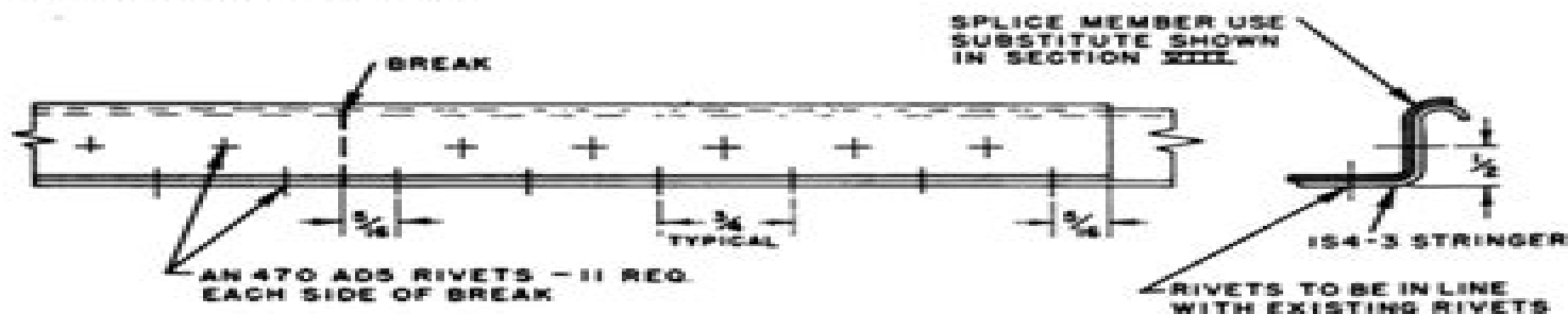
FIGURE 2-6. WING STRINGER REPAIRS
