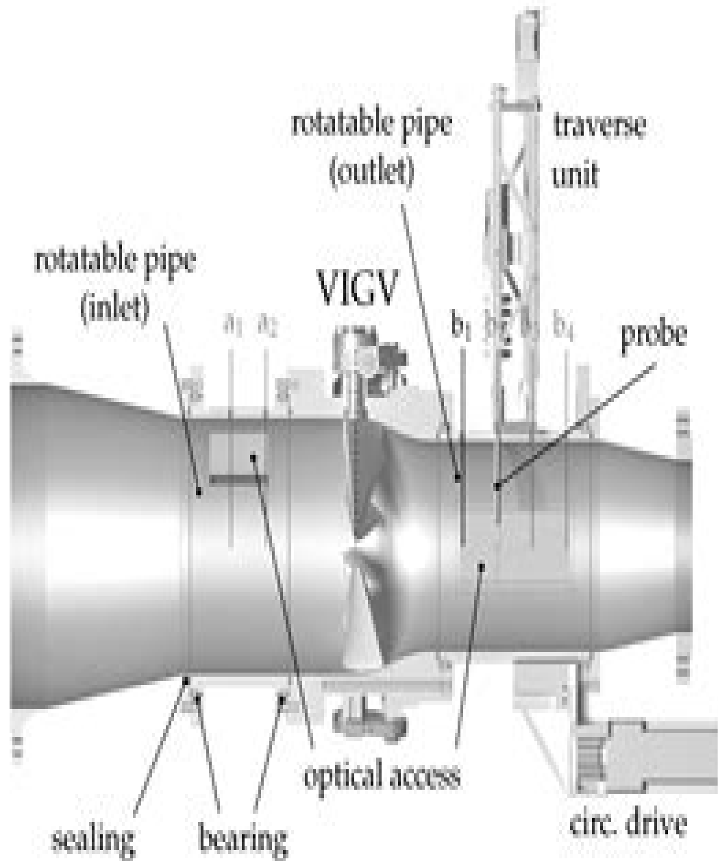
(b) Measurement section
