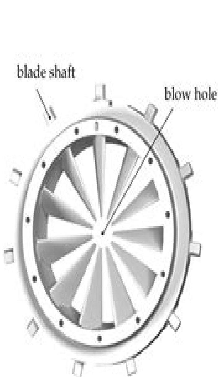
(a) Annular VIGV geometry
