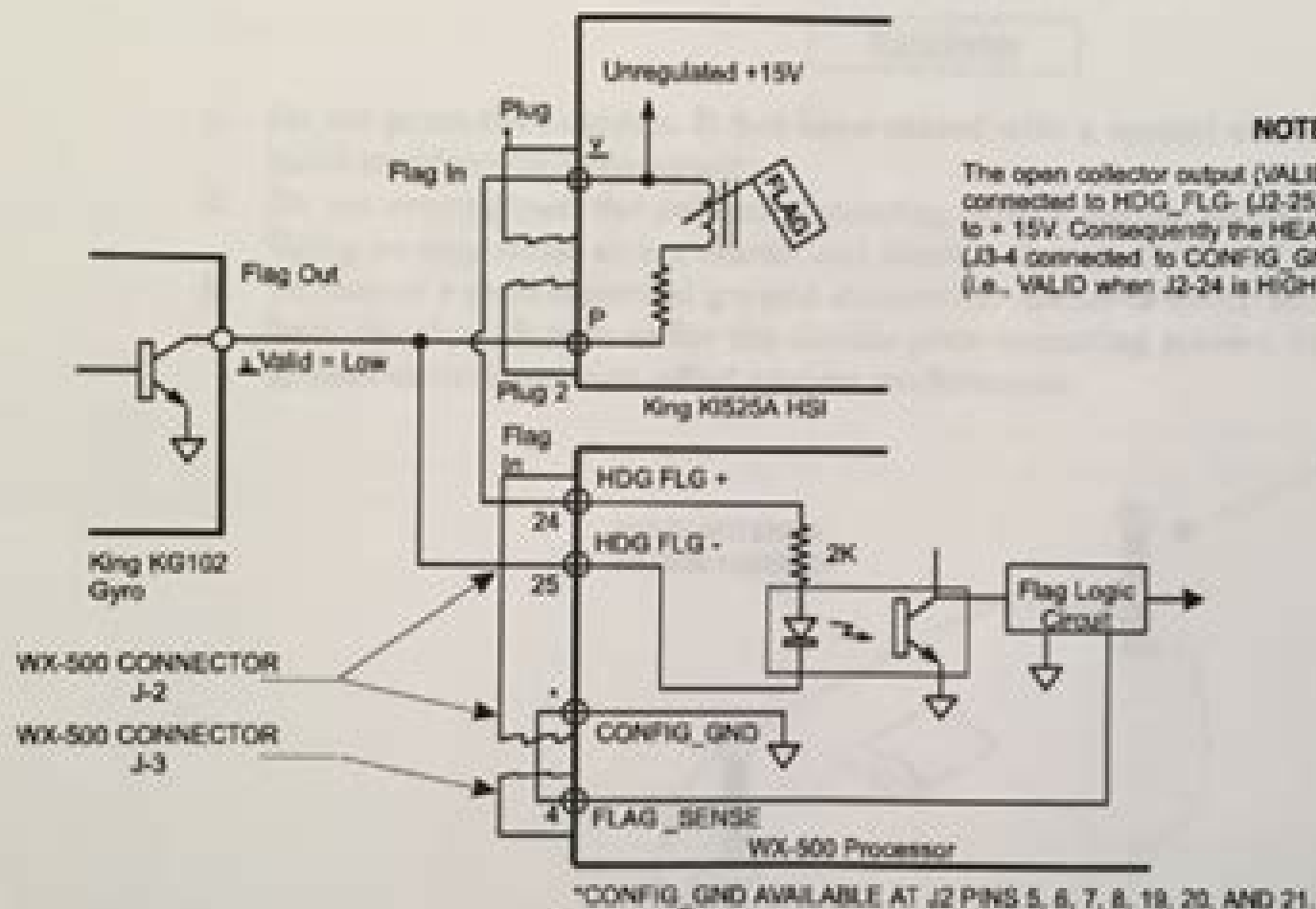
Figure 2-10. Heading Flag (KCS55) Connection
