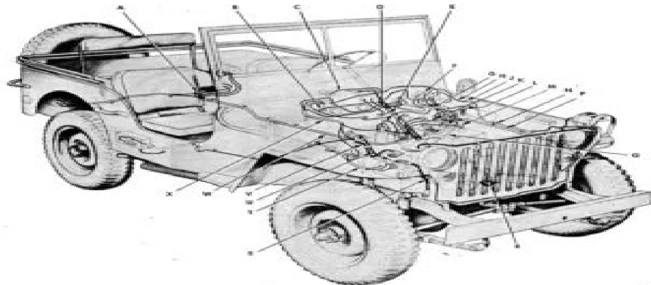
FIGURE 06-12—WIRING INSTALLATION
