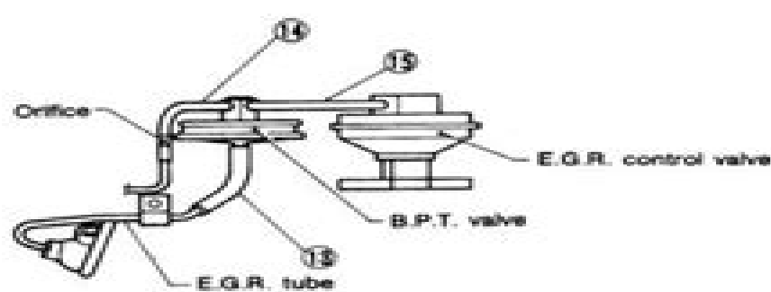
VIEW B
